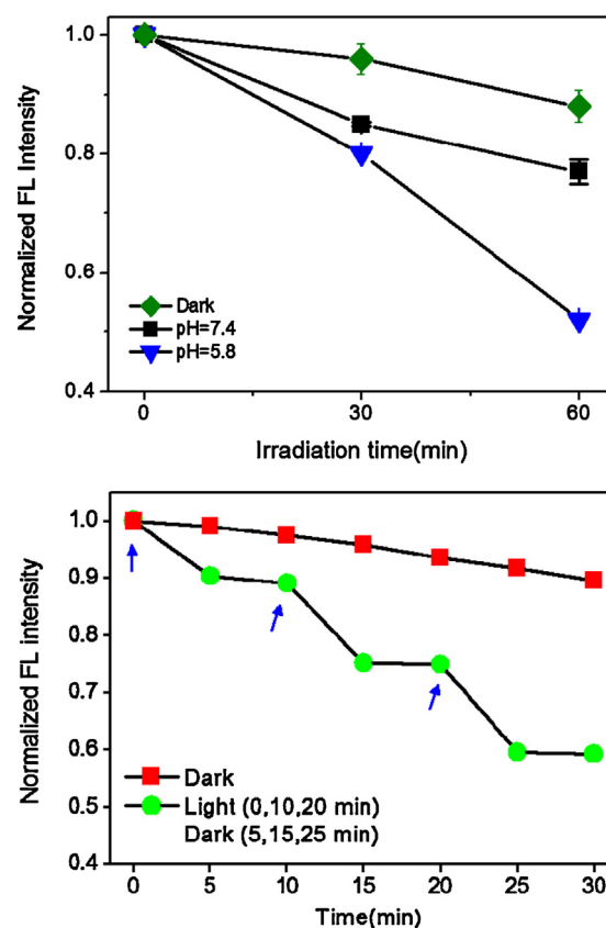
Fig. 7. (a) A pH-dependency of RhB releasing from hybrid hydrogel upon UV-light irradiation. (b) A stepped RhB releasing by alternating phototriggered and spontaneous processes. The hydrogel was irradiated with UV light at 0, 10, 20 min and exposed to darkness at 5, 15, 25 min.
